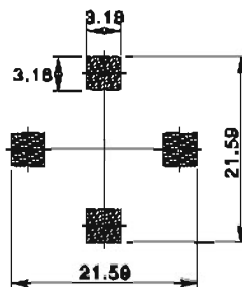
Recommended layout
