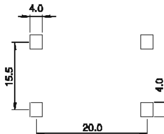
LAND PATTERNS
