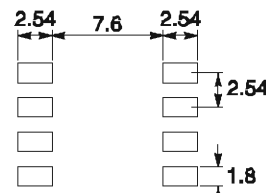
Layout recommendation
