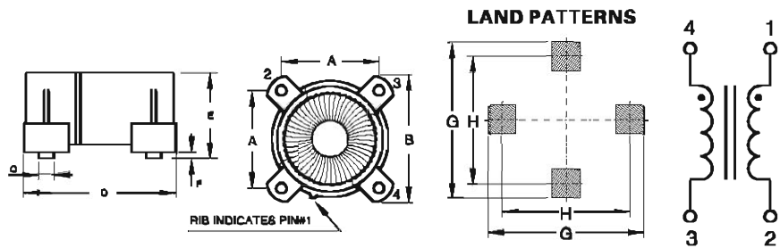
DIMENSIONS IN:mm
