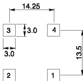
Recommended layout
