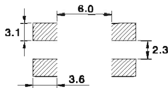
LAND PATTERNS
