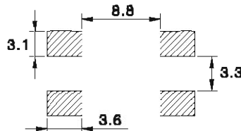
LAND PATTERNS
